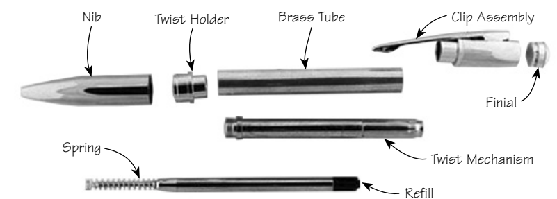
Yari pen parts.
